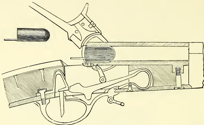
Demondion's Breech-loader.
